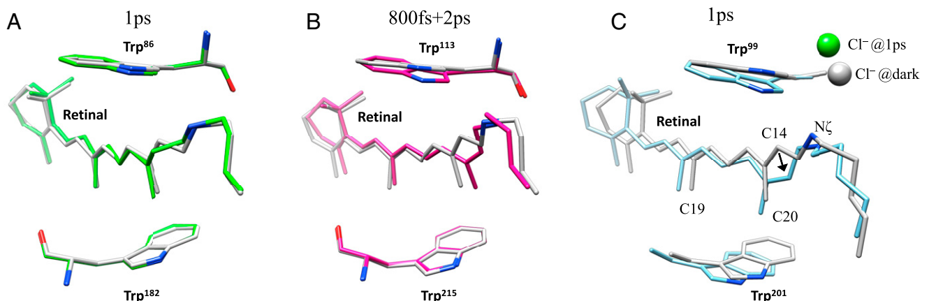
Fig. 6. Conformational change comparisons of the retinal and two nearby tryptophan residues in three rhodopsins. (A) bR (PDB 6GA4) (15); (B) KR2 (PDB 6TK7 for dark and 6TK5 for 800 fs + 2 ps) (16); and (C) CIR. In each panel, the corresponding dark-state structure is shown in gray as a reference.
